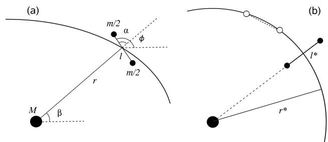
FIG. 1. (a) Instantaneous configuration of the system given by the generalized coordinates r , \beta , l , and \phi . The relative angle \alpha = \phi - \beta is indicated. (b) Two conservative synchronized configurations on a circular orbit of radius r^* . That of the black circles, corresponding to a solution of Eq. (3) with the spring stretched ( l^* > l_0 ), is stable. The other of white circles and the spring relaxed is unstable.
